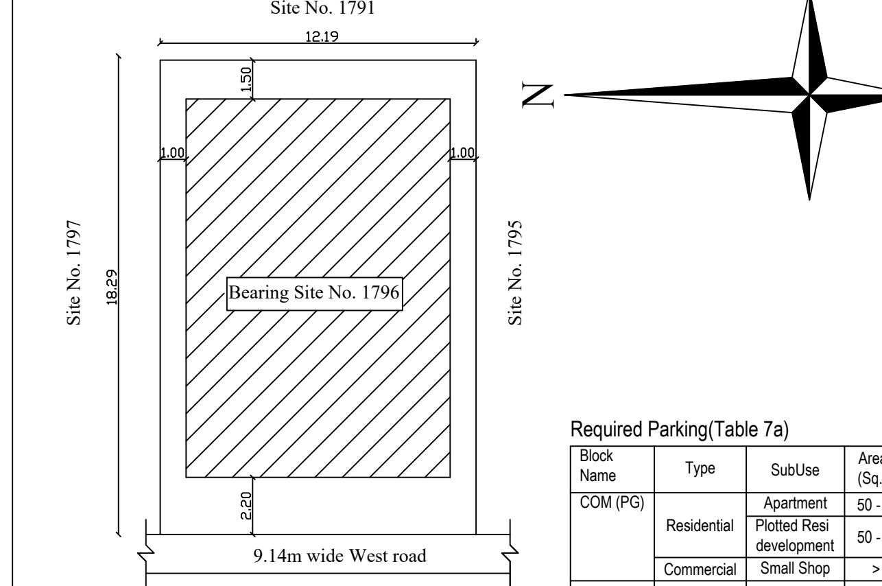
SITE PLAN
