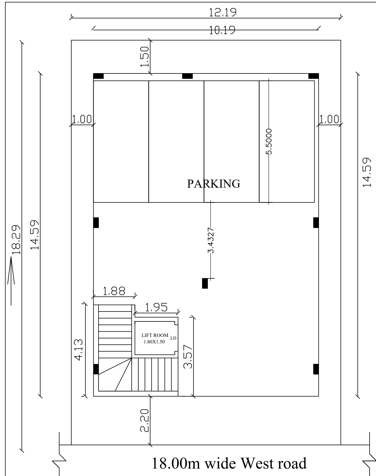
PROPOSED STILT FLOOR PLAN
