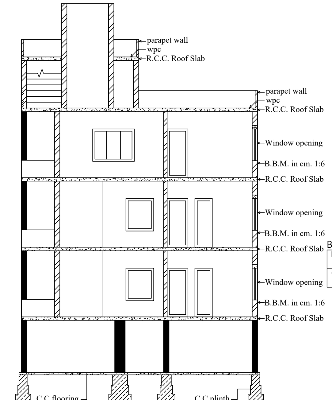
SECTION
